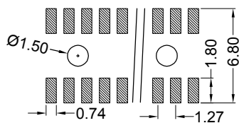
Recommended P. C. B LAYOUT General Tolerance ±0.05
