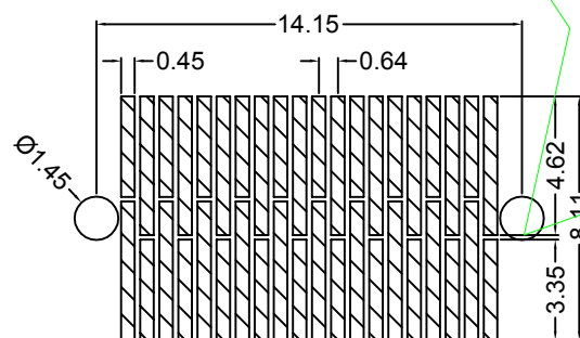
General Tolerance \pm 0.05
