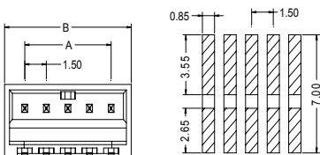
Recommend PCB Layout
