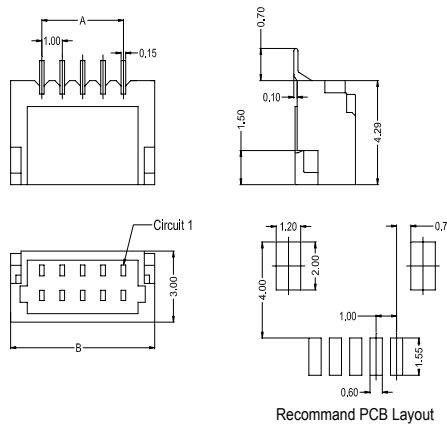
Recommad PCB Layout
