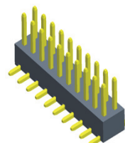
P143-12XXXXMXXX1 L=B+4.5+(W-2.54)/2
