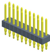
P125-12XXXXXXSXXX1 L=A+B+2.5
