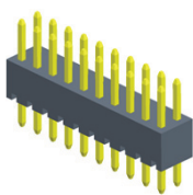
P143-12XXXXXSXXX1 L=A+B+4.3
