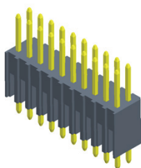
P174-12XXXXXSXXX1 L=A+B*7.4
