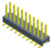
P125-12XXXXM1 L=B+2.5+D+(W-2.54)/2
