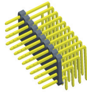
P2XX-14XXXXXRXXXX1 L=A+B+D+H+1.0
