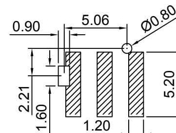
Recommended P.C.B Layout T=1.70mm General Tolerance ±0.05
