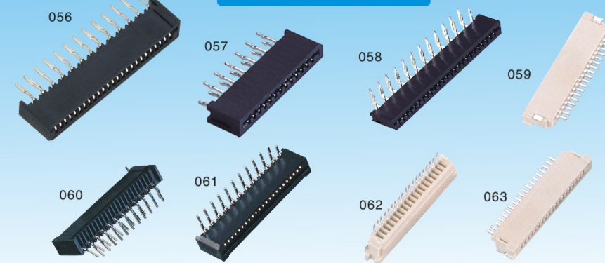
1.25mm/Pitch FPC
