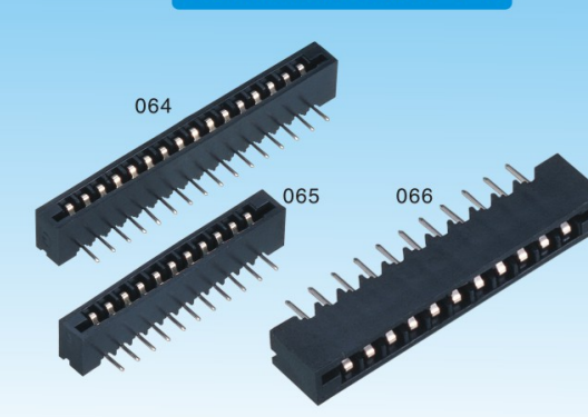
2.54mm/Pitch FPC
